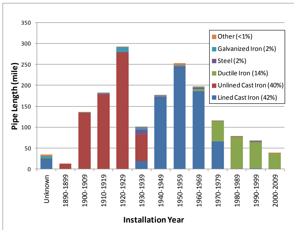
Figure 5-2. Type of Material and Decade of Installation for SPU's Distribution System Watermains
