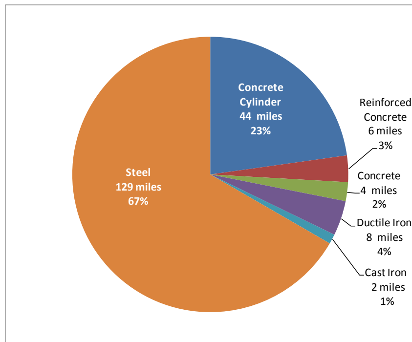
Figure 4-1 Breakdown of Transmission Pipeline Material
