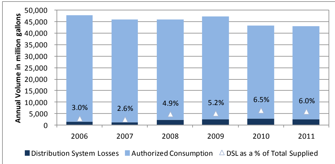
Figure 5-1. Distribution System Leakage
