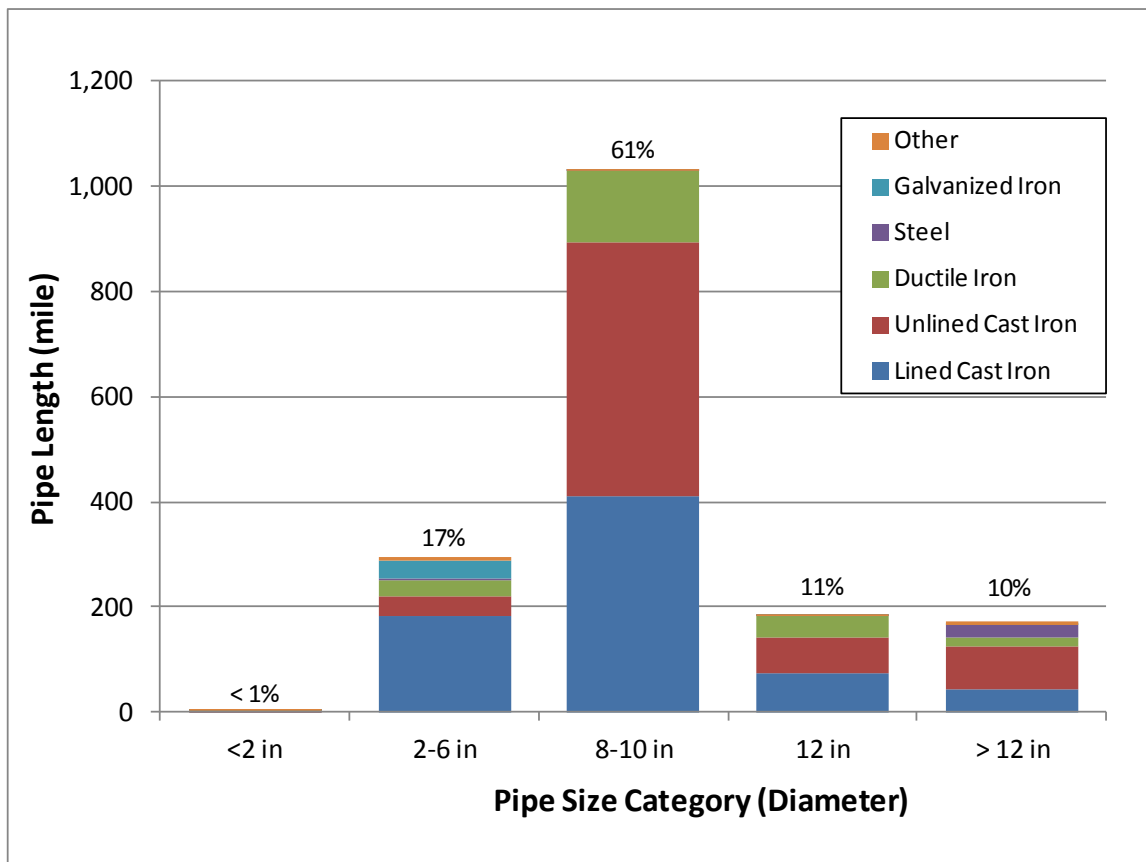
Figure 5-3. Pipe Diameter and Material Types for SPU's Distribution System Watermains
