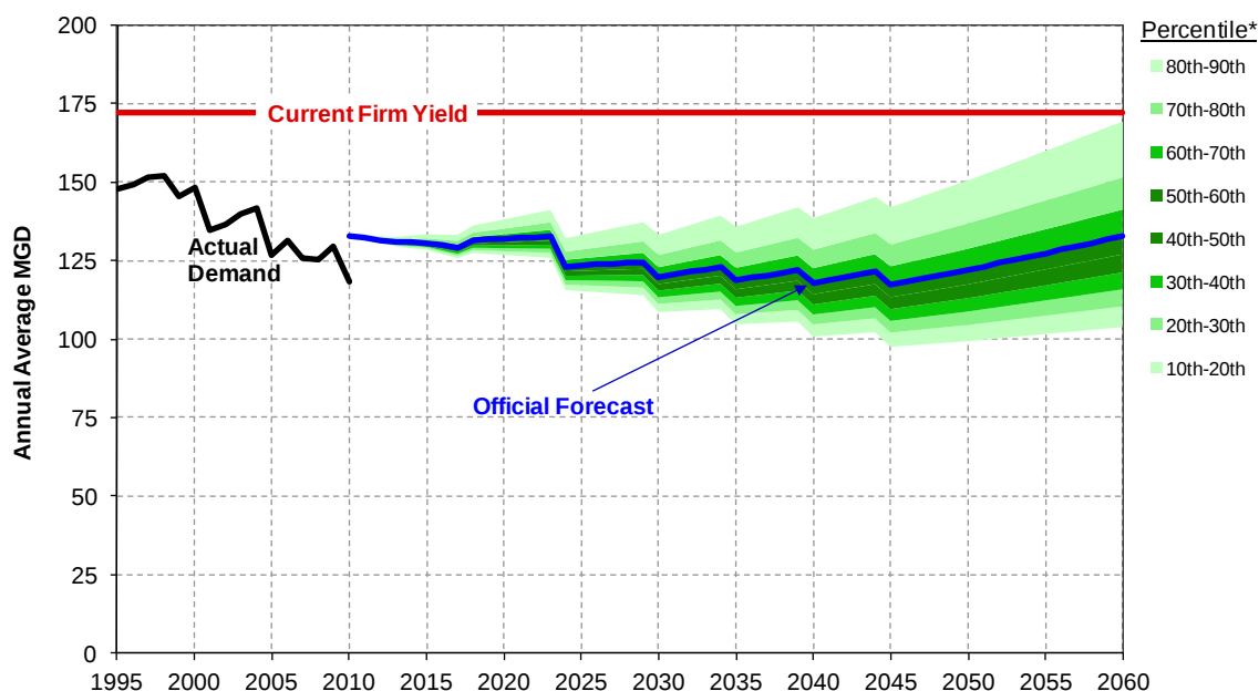
Figure 2-6. Uncertainty in Water Demand Forecast 2
