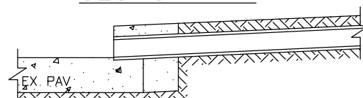
SECTION B-B
