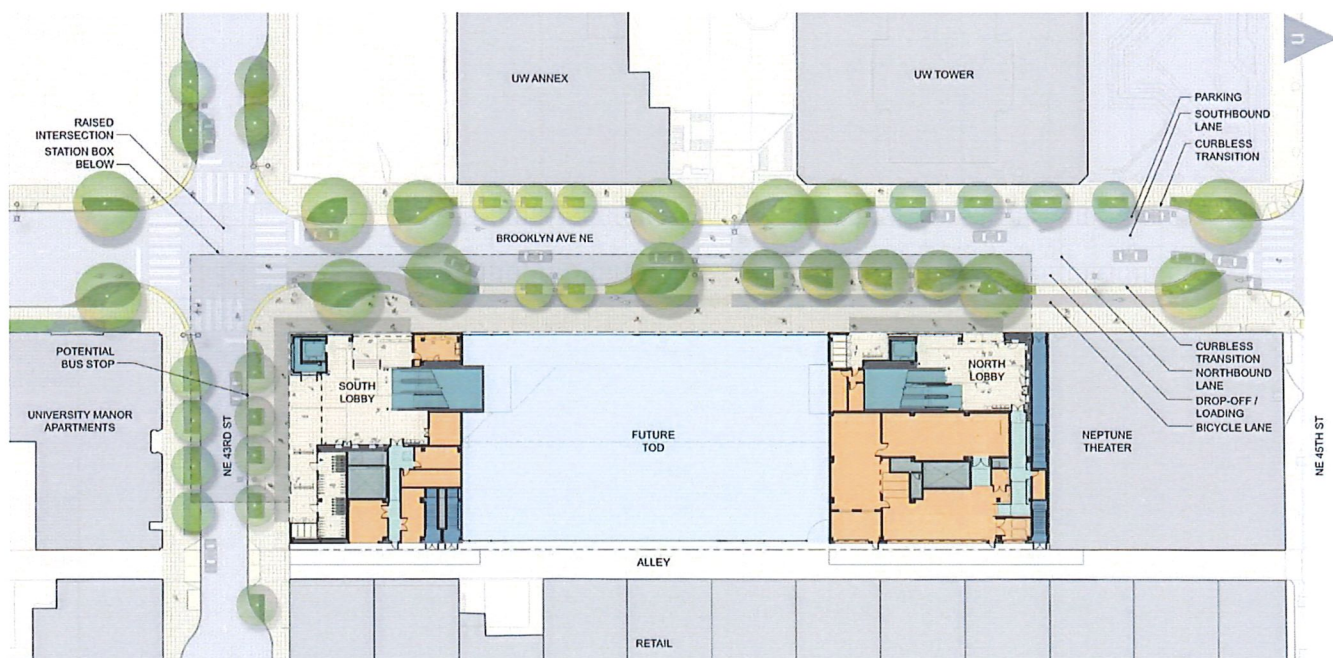
Figure 9. U District station site plan.
