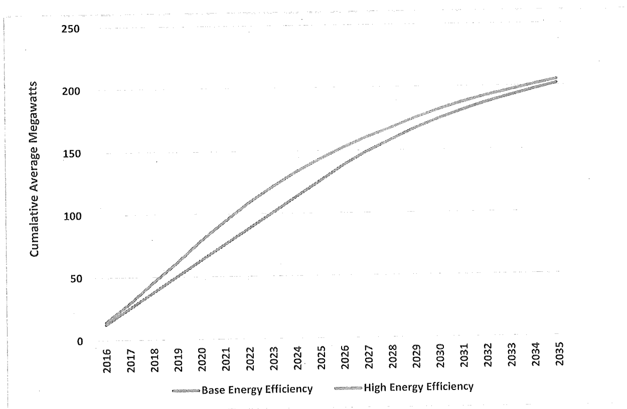
Figure 6. Base and High achievement of Energy Efficiency (2015 Conservation Potential Assessment)
