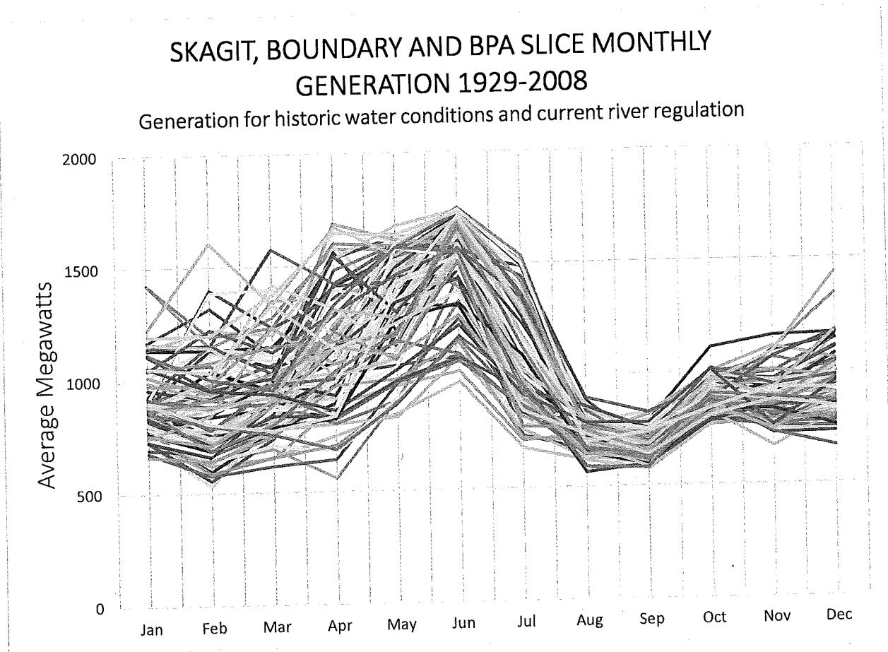
Figure 3. Seasonal and Annual Variability in City Light Hydro Resources
