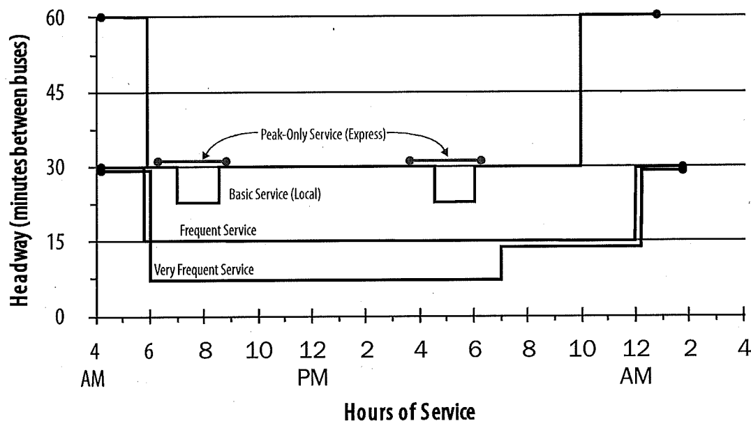
FIGURE 4-4 SERVICE TARGETS FOR THE FREQUENT TRANSIT NETWORK
