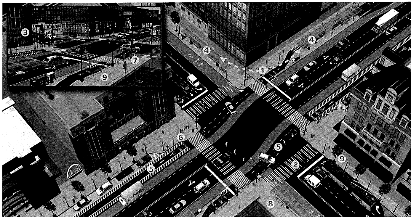
FIGURE 5-3 DESIGN ELEMENTS AT CONCEPTUAL PRIORITY ACCESS NODE
