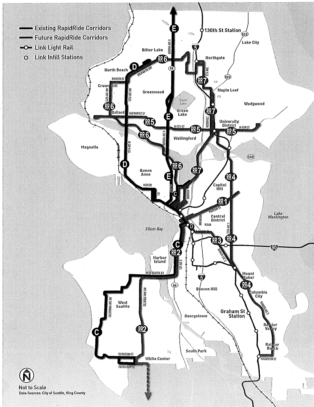
FIGURE 3-7 EXISTING AND PROPOSED RAPIDRIDE CORRIDORS
