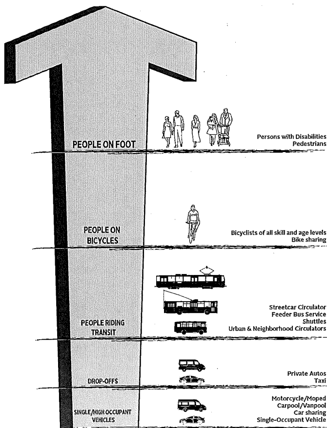
FIGURE 5-7 ACCESS HIERARCHY
