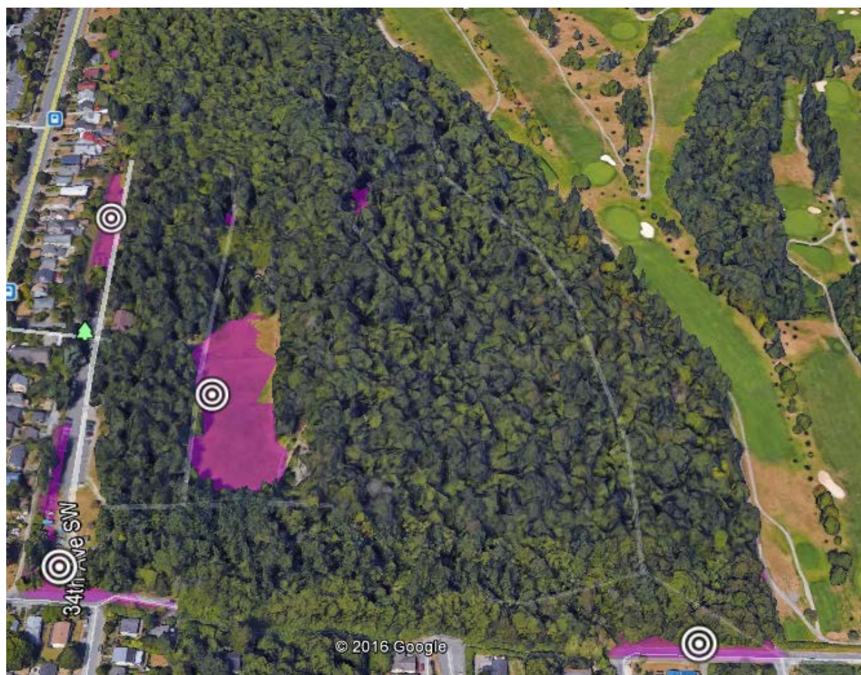
Figure 24: Camp Long High-Level Wi-Fi Network Design Map
