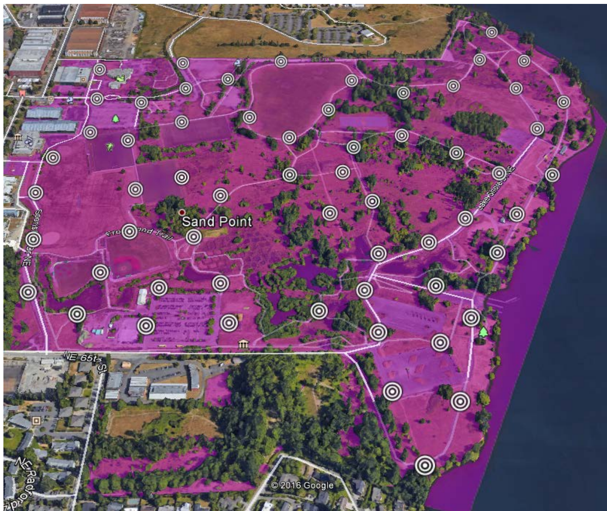
Figure 22: Walter E. Magnuson Park High-Level Wi-Fi Network Design Map
